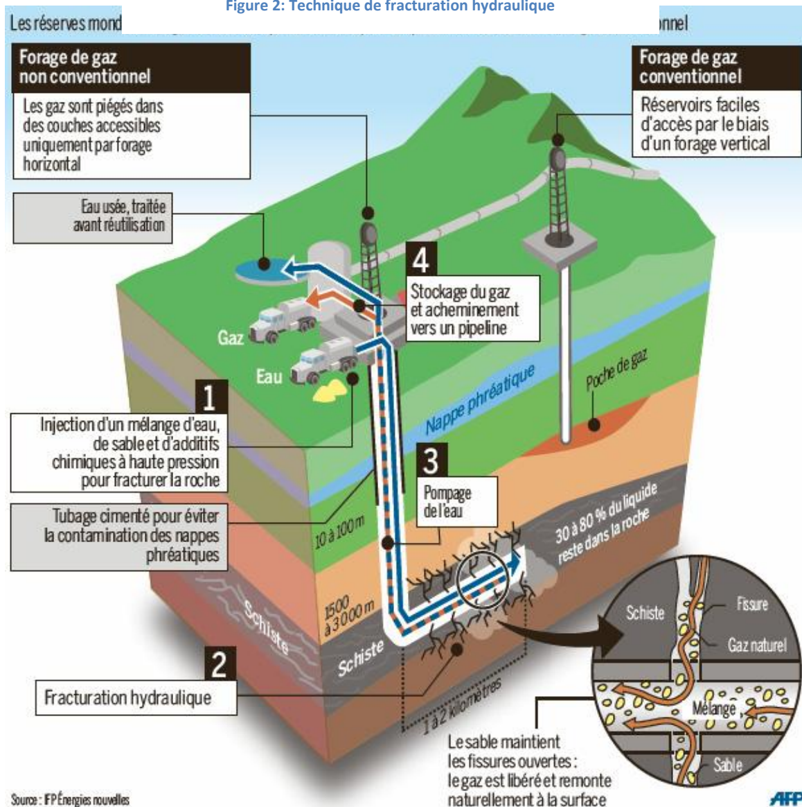
Figure 2: Technique de fracturation hydraulique
